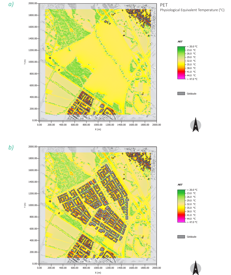
Figure 32. Example of numerical 3D modeling simulations to evaluate the influence of building layouts on the local microclimate.
