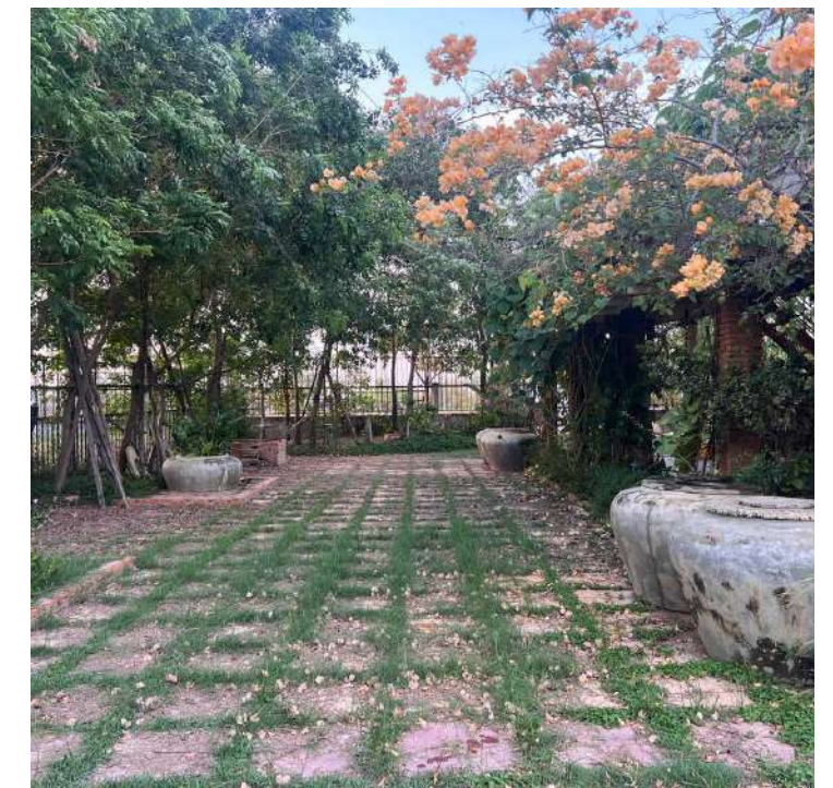
Figure 16. Example of the application of permeable pavement in a parking area in urban Cambodia. Source: Tep Makathy (2025).
